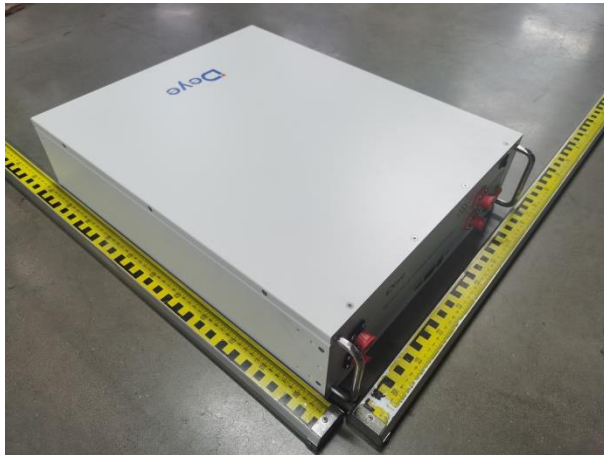
电池/ Battery(SE-G5.1Pro-B 51,2V 100Ah 5,12kWh)
