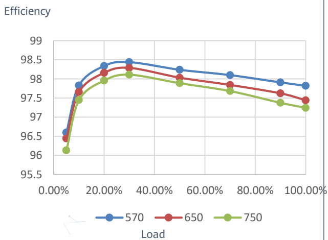
Efficiency Curve
