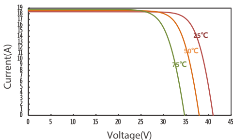
IV Curves of JT600SHK at different Temp
