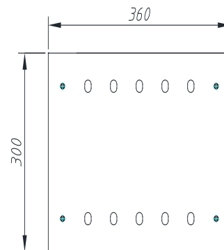
Optional: Post Mounting Plate
